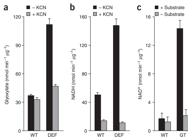
Figure 2 Activities of the bacterial enzymes in chloroplast extracts. Chloroplasts were isolated from descendants of transgenic lines and wild-type (WT) plants. Genotypes are described in the main text. (a) Glycolate dehydrogenase assay. (b) D-lactate dehydrogenase assay. (c) Coupled assay for glyoxylate carboxyligase and tartronic semialdehyde reductase. DEF, plants overexpressing subunits D, E, and F of E. coli glycolate dehydrogenase; GT; plants overexpressing glyoxylate carboxyligase and tartronic semialdehyde reductase. Controls are indicated in the figure. Each data point is based on at least three independent measurements. Error bars indicate s.e.m.
