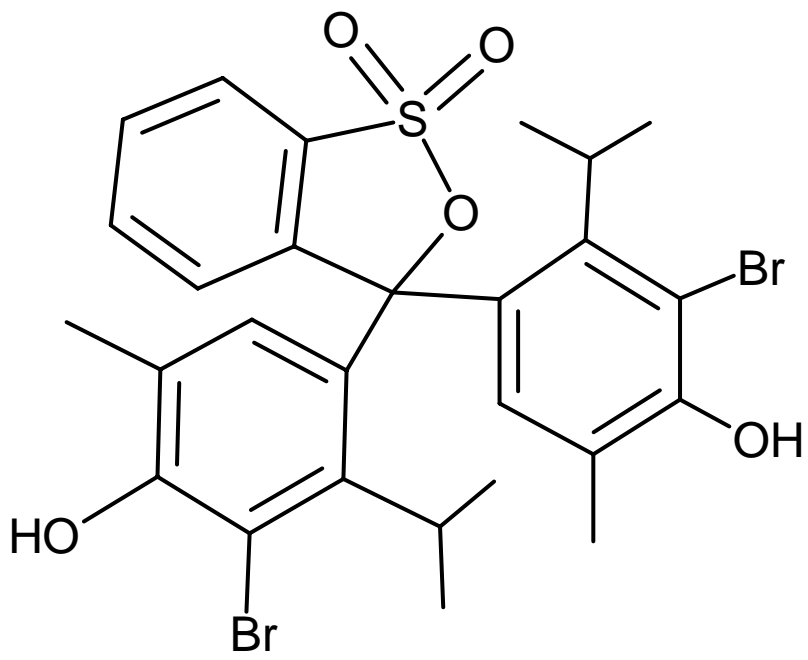
Bromothymol blue (pH 6.0-7.6)
