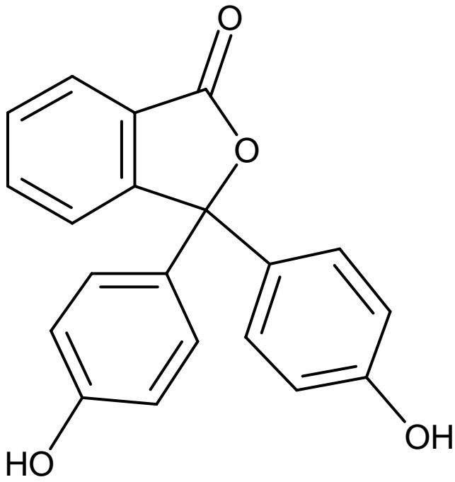
Phenolphthalein (pH 8.0-9.6)
