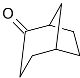
Bicyclo[3.2.1]octan-2-one
