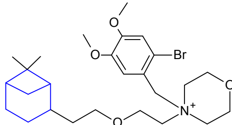
AND Enantiomer
