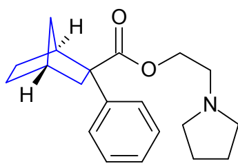
Bicyclophenamin Spasmolytic
