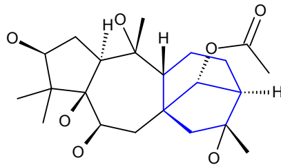
Acetylandromedol Antihypertensive
